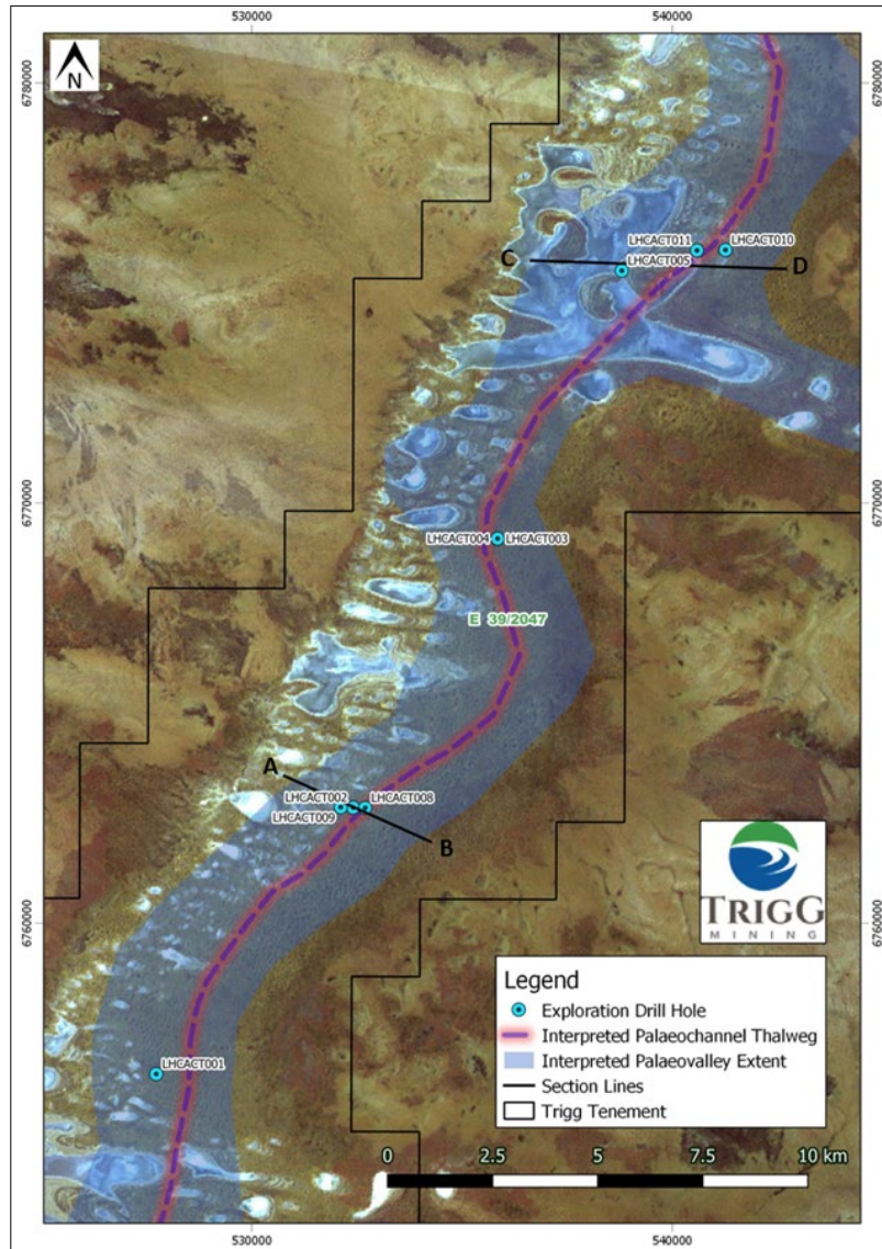
Figure 5: Drilling transects completed at Lake Hope Campbell
